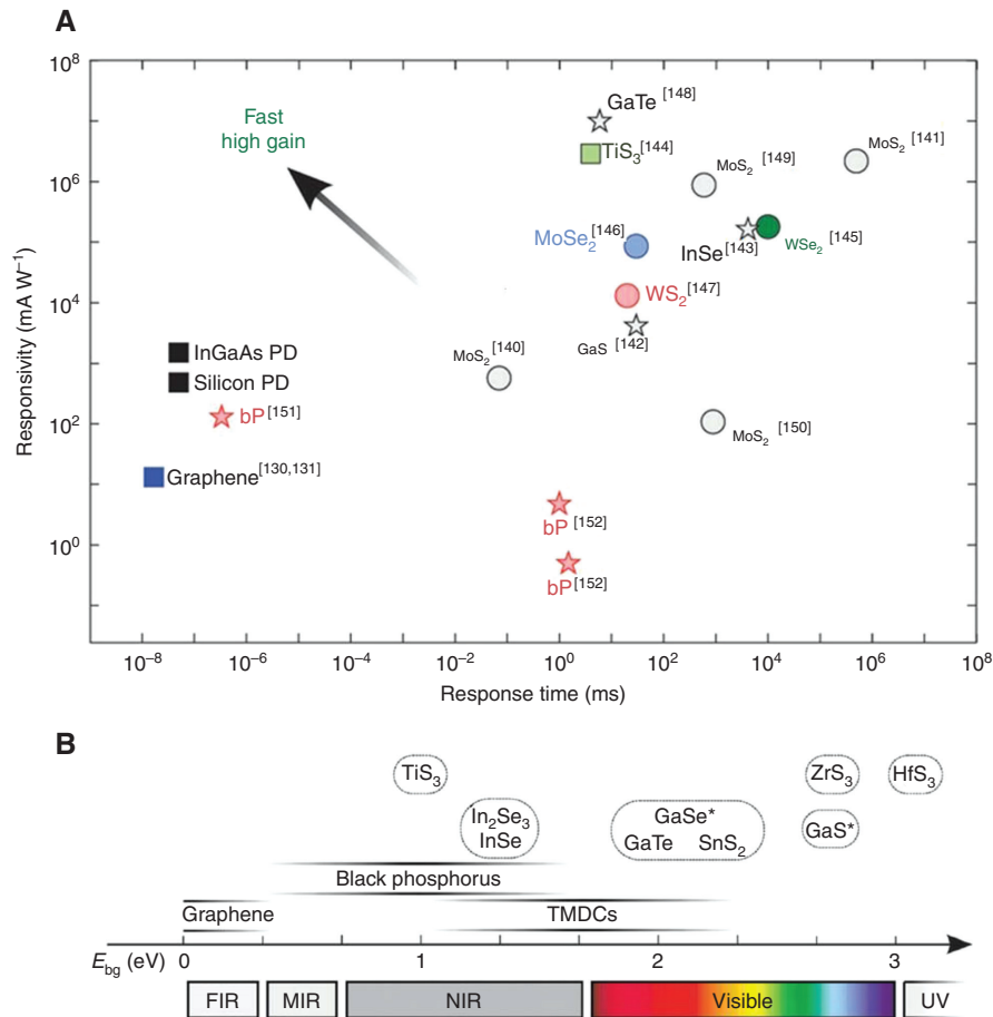
Figure 8: Summarization of important characteristics for detection application using different 2D materials.
