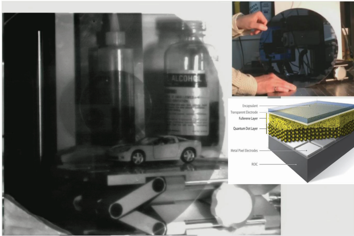
Figure 9: An image from the PbS CQD-based focal plane array (FPA) camera operating in the SWIR band. The CQD-based camera can see through a silicon wafer. The first inset shows the image taken using a normal visible camera. Second inset image is the PbS CQD-based focal plane array (FPA) structure [162].
