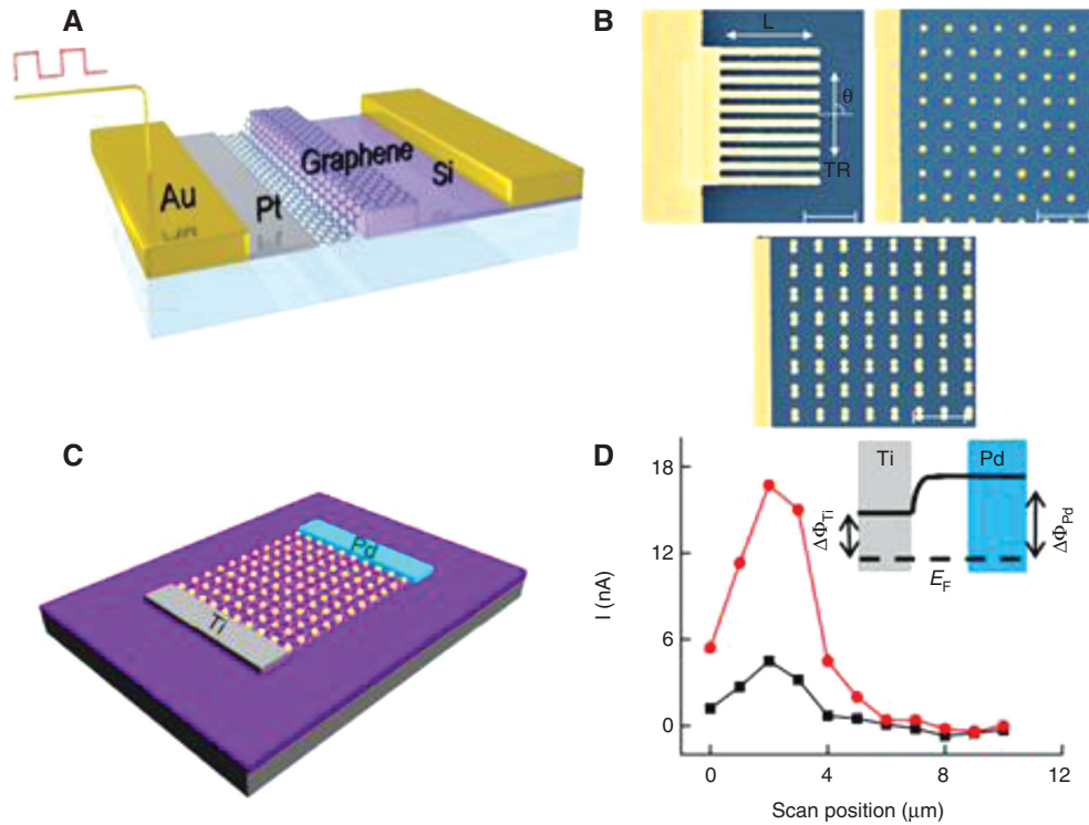
Figure 14: Photodetection enhancement by metallic plasmonics and graphene. (A) Schematic of a monolayer graphene sheet is on top of a silicon bus waveguide [202]. (B) Different metallic structure to enhance the performance of graphene-based device. Scale bar = 1 \mu\text{m} [203]. (C) Schematic diagram of a graphene-based photodetector with asymmetric metal contacts (Ti and Pd) decorated with Au nanostructures. (D) Photocurrent profile with laser scanning from outside of the Ti electrode (black line: normal graphene device; red line: plasmon resonance-enhanced graphene device). The inset shows the band profile of the asymmetric metal-contacted graphene photodetector [204].
