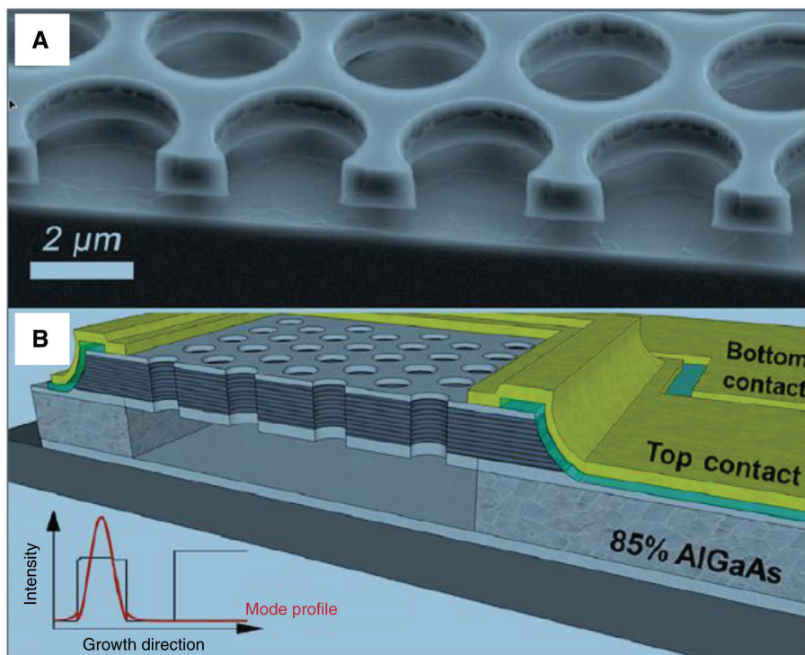
Figure 12: PCS-QWIP design.
