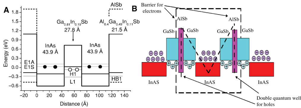
Figure 4: Schematic diagram of W- and M-T2SL LWIR photodiodes. (A) Band profiles of W-T2SL [58] and (B) p-doped M-T2SL structure [59].
